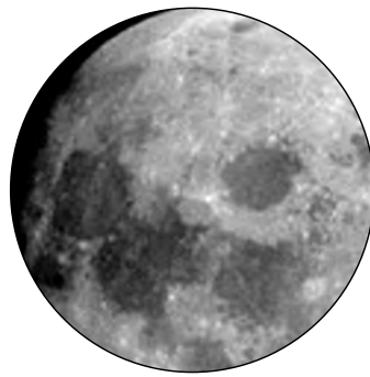
The Moon
