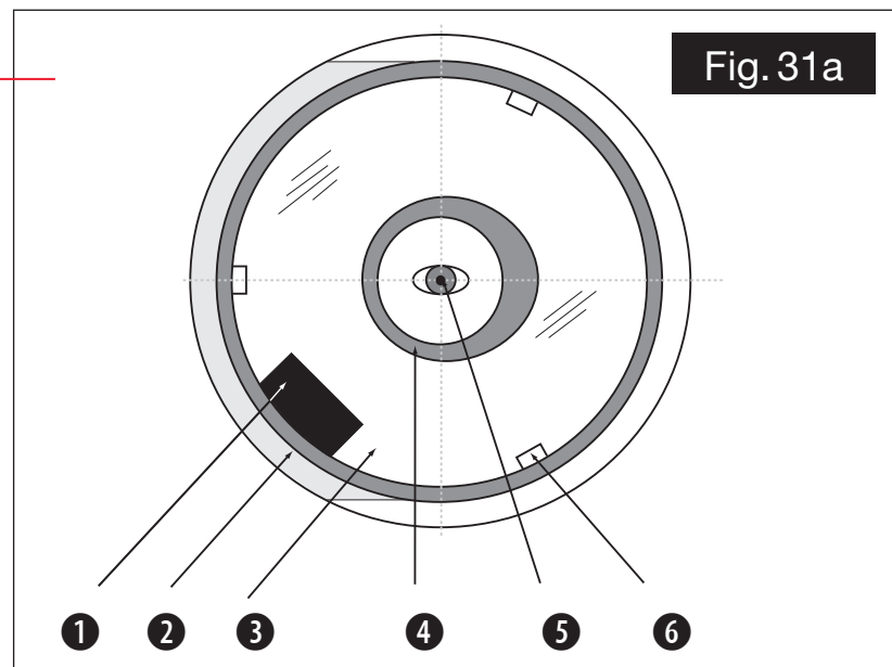
Fig. 31a shows a correctly collimated Newtonian telescope, as it appears when viewed through the focuser with the eyepiece removed.
