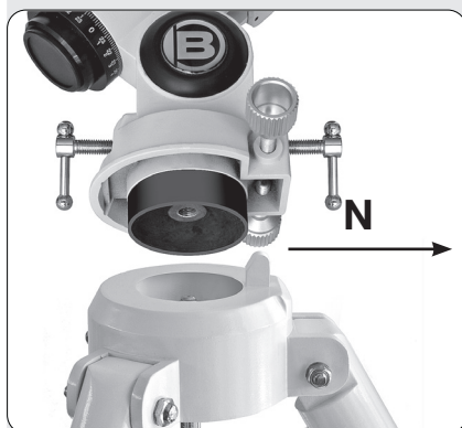
Fig. 2d: installing the mounting on the EXOS-1 tripod.
